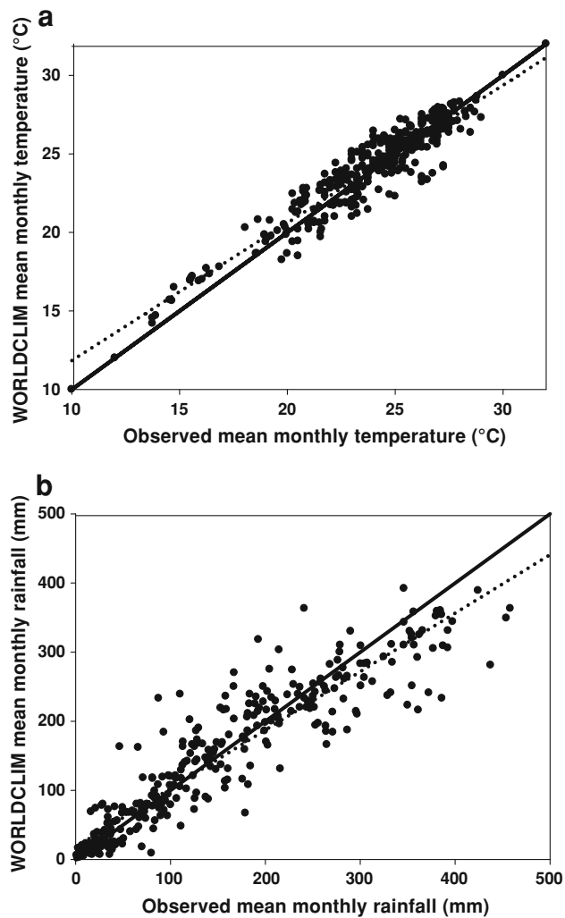
Fig. 3 Interpolated current ( \sim 1950 – 2000 ) a mean monthly temperature and b monthly rainfall from the WORLDCLIM database compared to observed values at 26 sites in Timor Leste for which data is available for 20 years from 1954 to 1974. Solid line The 1:1 relationship and dotted line the fitted linear regression
