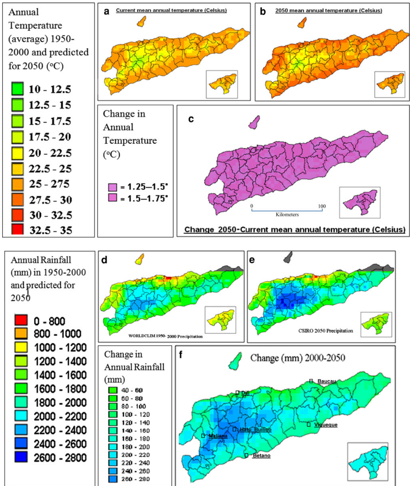
Fig. 4 The current (~1950–2000) (a, d), predicted for 2050 (b, e) and the difference between 2050 and current (c, f) mean annual temperatures (a–c) and rainfall (d–f) for Timor Leste. The inset is for the Timor Leste enclave of Oecussi in West Timor. The values of temperature change have been grouped into one band and colour (1.25–1.75°C). This was because there was no spatial pattern or
