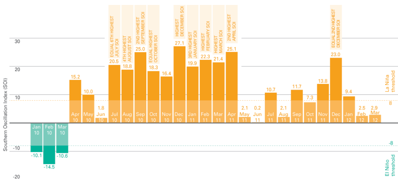
Monthly SOI values for the 2010–11 and 2011–12 La Niña events – numerous record and near-record values for that particular month are indicated
