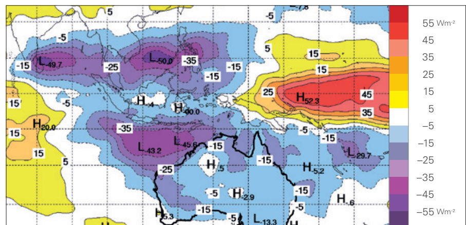
Outgoing long-wave radiation (OLR) anomalies over the greater Australasian region for summer 2010–11. Negative anomalies (blue and purple colours) indicate increased cloudiness and less heat lost to space, while positive anomalies (yellow and red colours) indicate reduced cloudiness. The widespread cloud over the Australia–Indonesia region during the summer is clearly shown.
