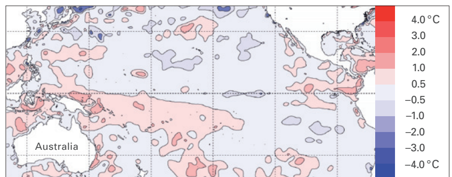
May 2010 – between the end of El Niño and the start of the 2010–11 La Niña; relatively neutral state of the ocean
