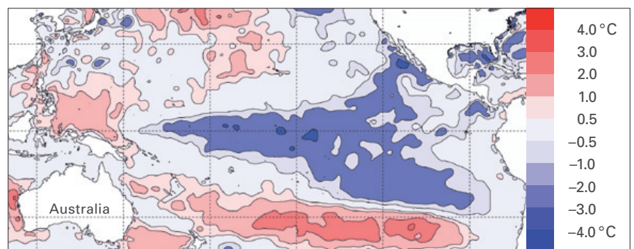
January 2011 – peak of the 2010–11 La Niña; cooler than normal sea surface temperatures in the central and eastern Pacific
