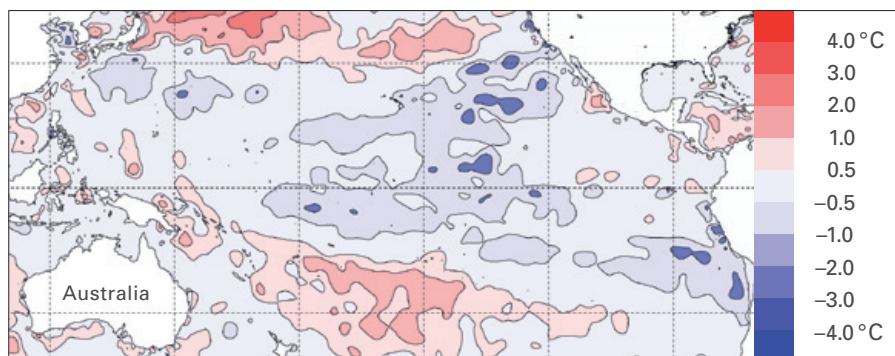
September 2011 – cooling in the central Pacific as the La Niña re-forms
