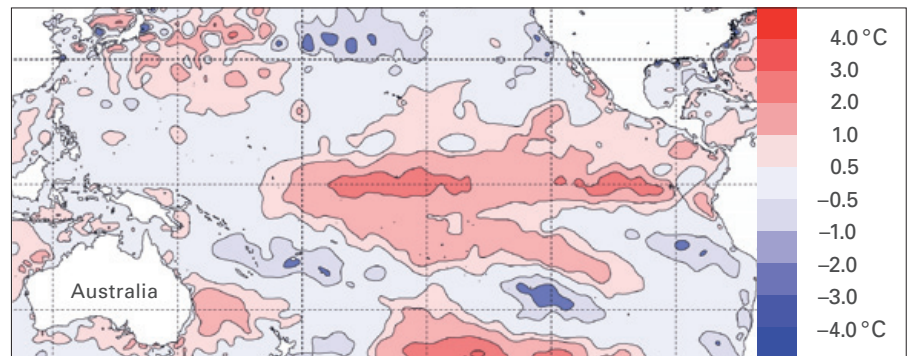
December 2009 – peak of the 2009–10 El Niño; warmer than normal sea surface temperatures in the central and eastern Pacific
