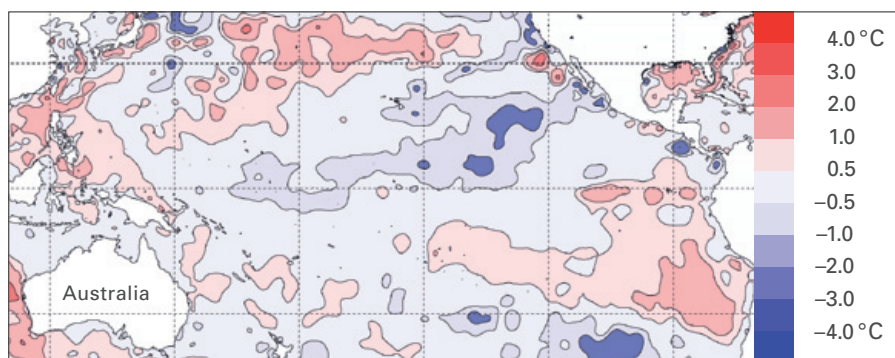
March 2012 – 2011–12 La Niña has declined; ocean temperatures in the Pacific approach neutral
