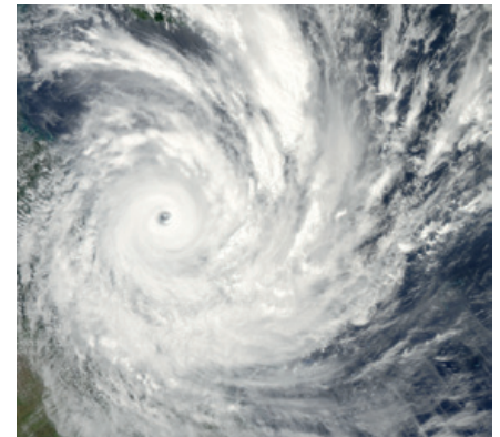
Tropical cyclone Yasi as it approached the Queensland coast just south of Cairns, captured by the Moderate Resolution Imaging Spectroradiometer (MODIS) on NASA's Aqua satellite, 2 February 2011
