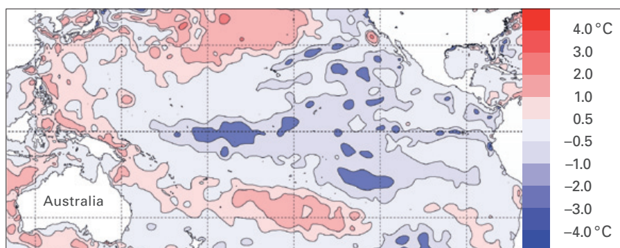
December 2011 – peak of the 2011–12 La Niña; cooler than normal central and eastern Pacific, but not as cool as at the 2010–11 La Niña peak
