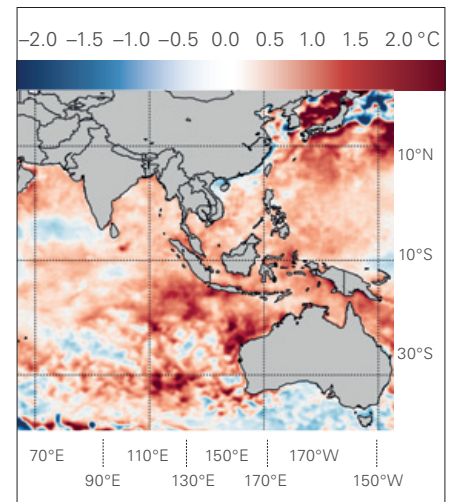
October 2010 monthly sea surface temperature anomalies (°C) in the Indian Ocean show much warmer than usual waters in the eastern end of the dipole near Australia. (Anomalies are calculated with respect to the Reynolds climatology for 1971–2000 from the National Climatic Data Center.)
