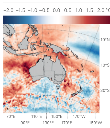
Sea surface temperature anomalies (°C) in the Australian region, for the period May 2010 to April 2011
